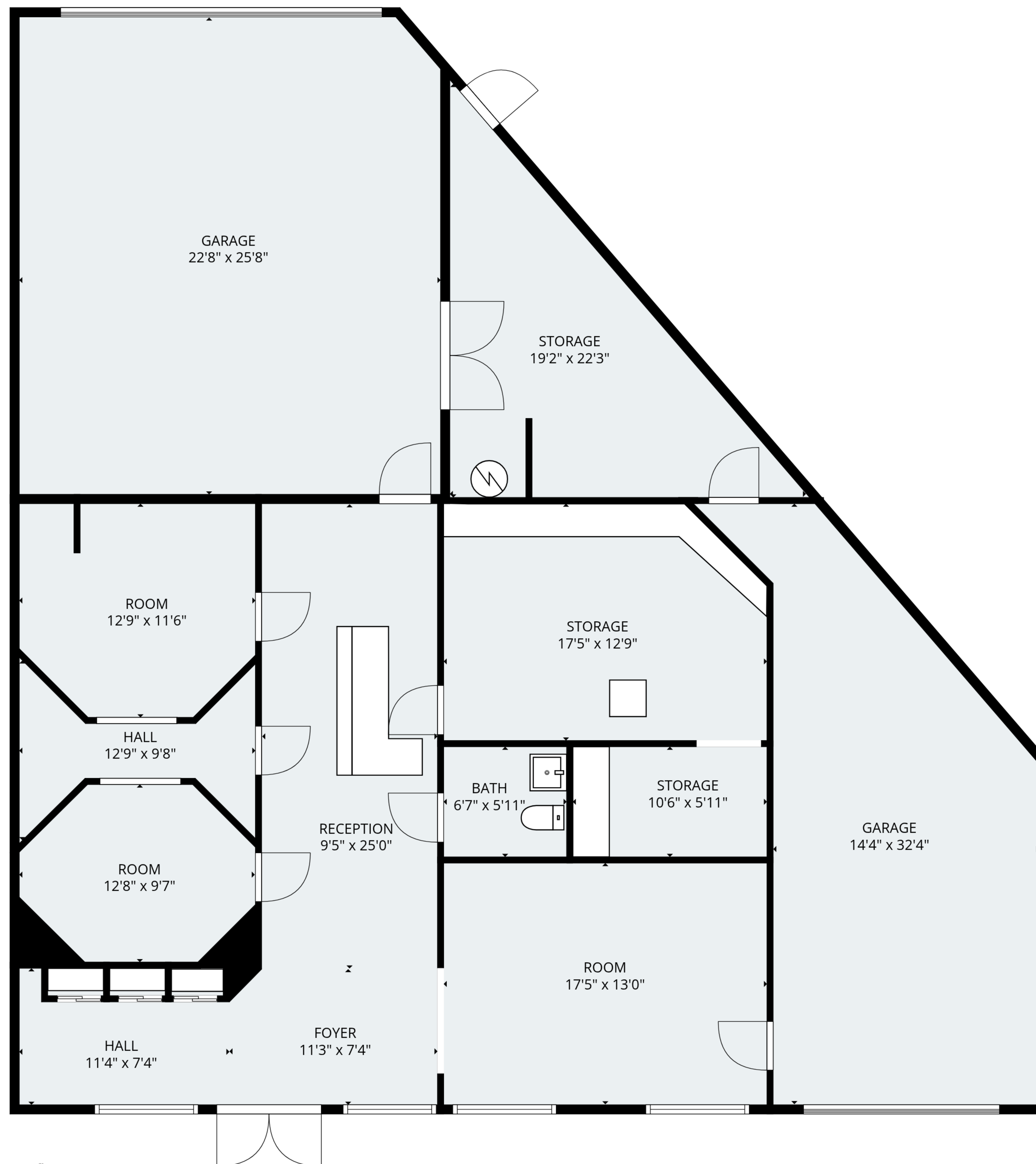
1st floor
