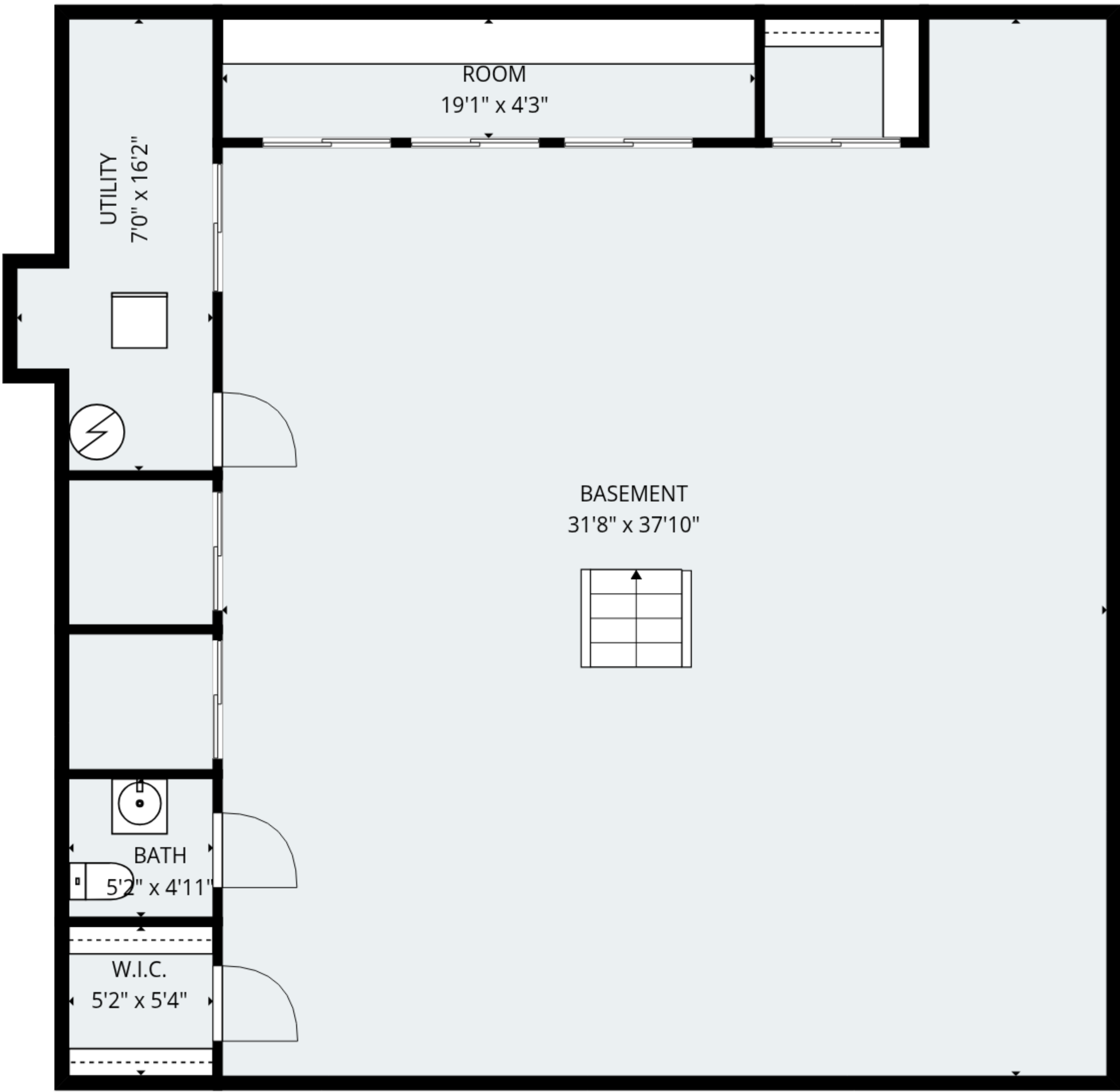
FLOOR 1
