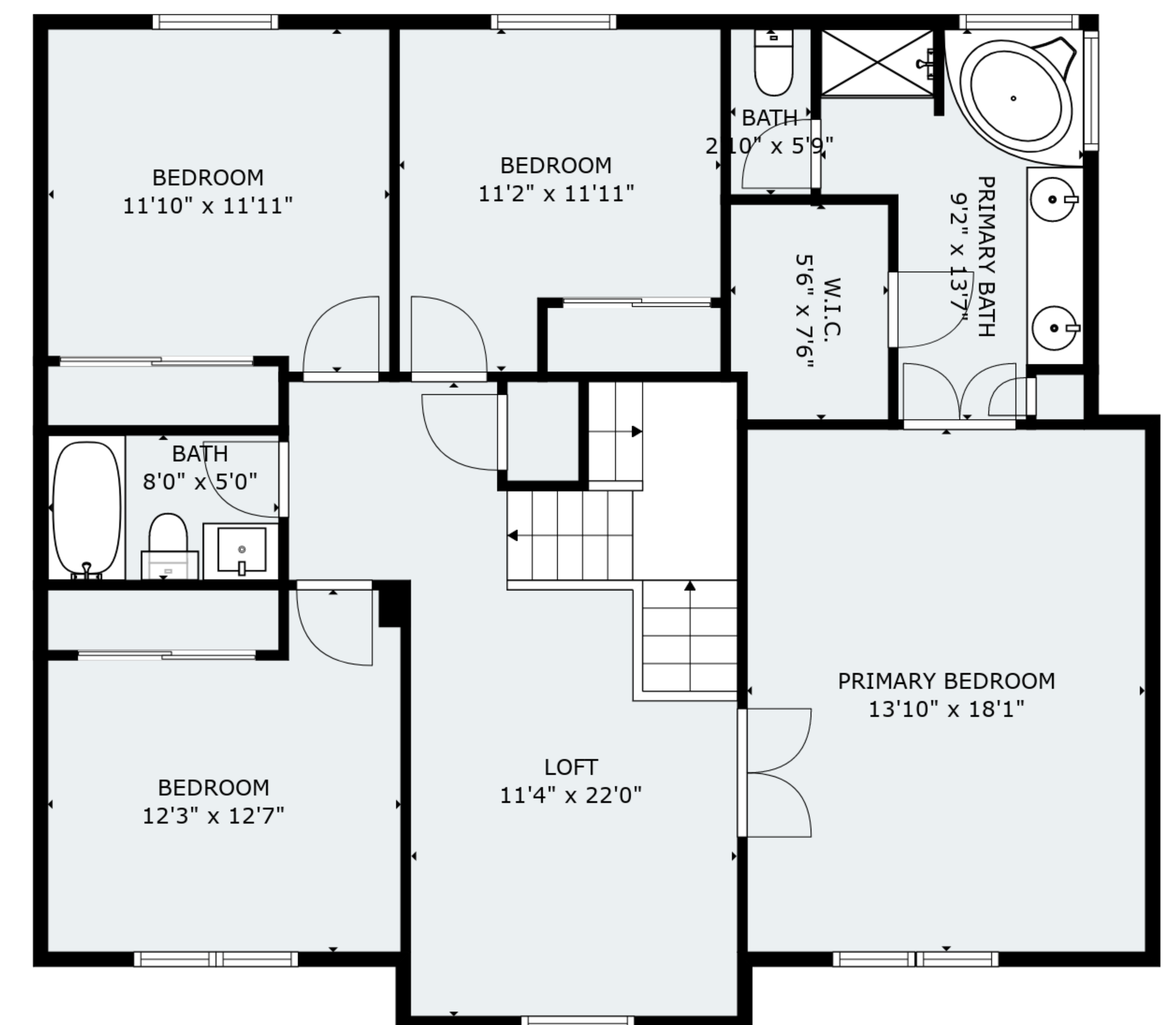
FLOOR 3
