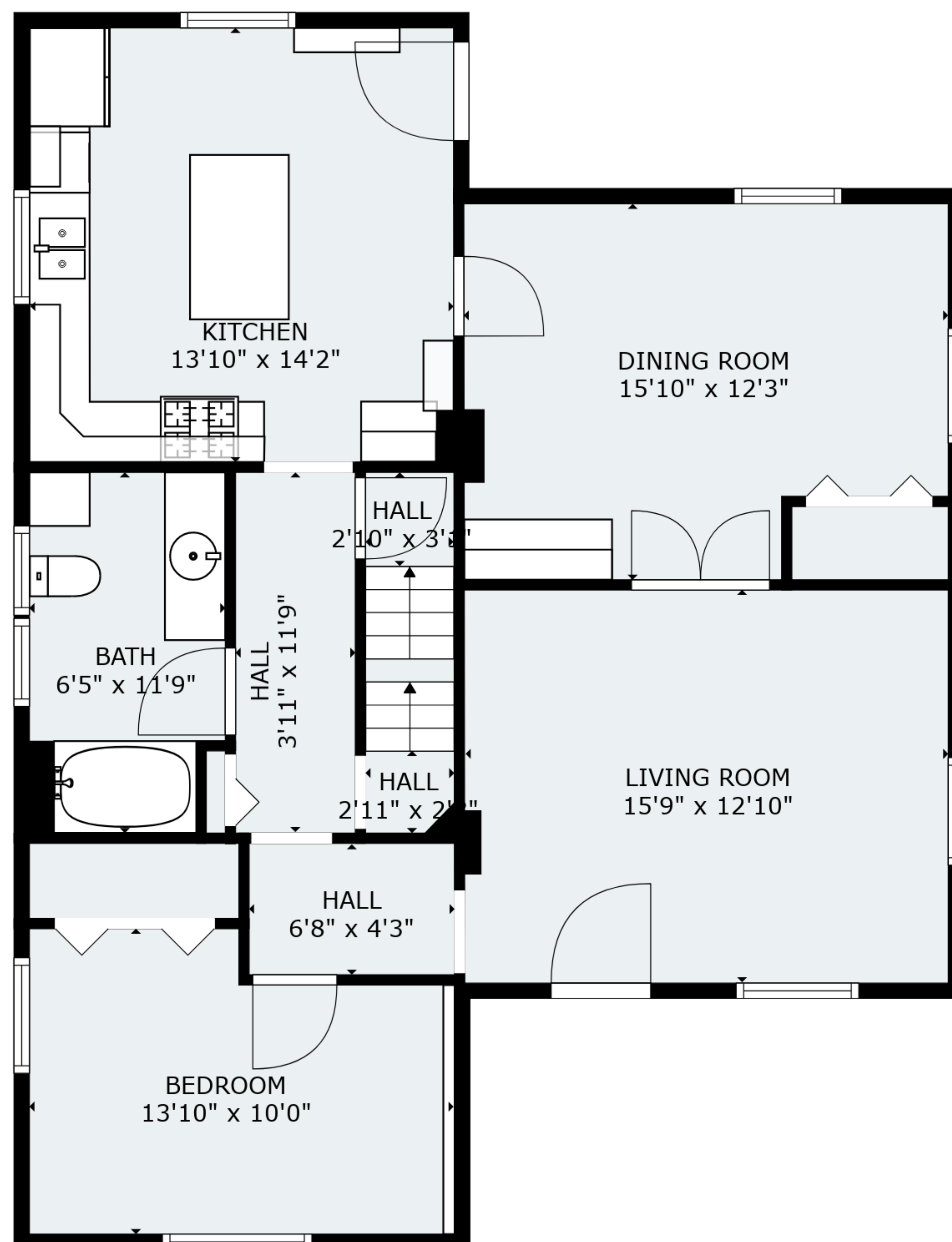
FLOOR 2
