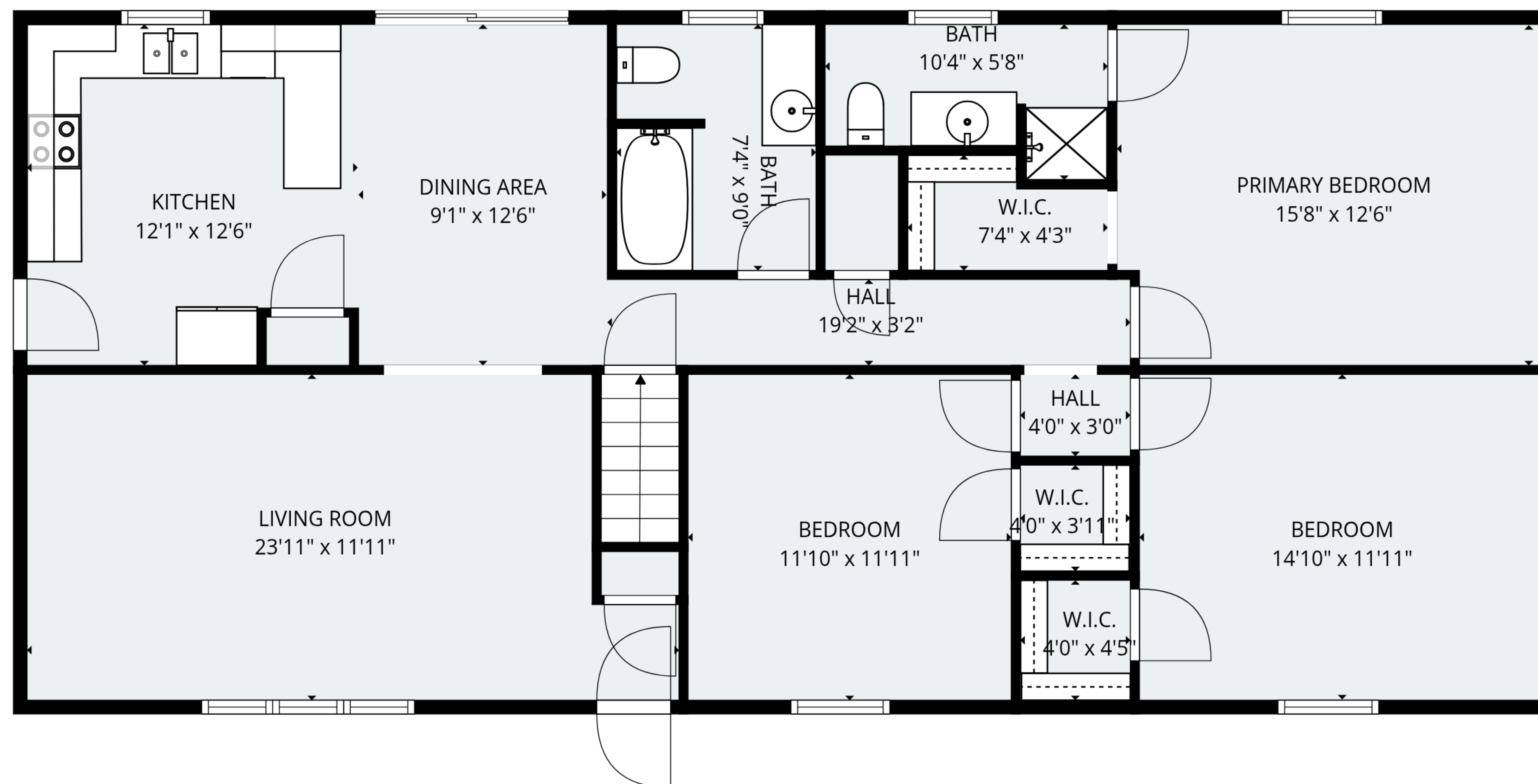
FLOOR 2
