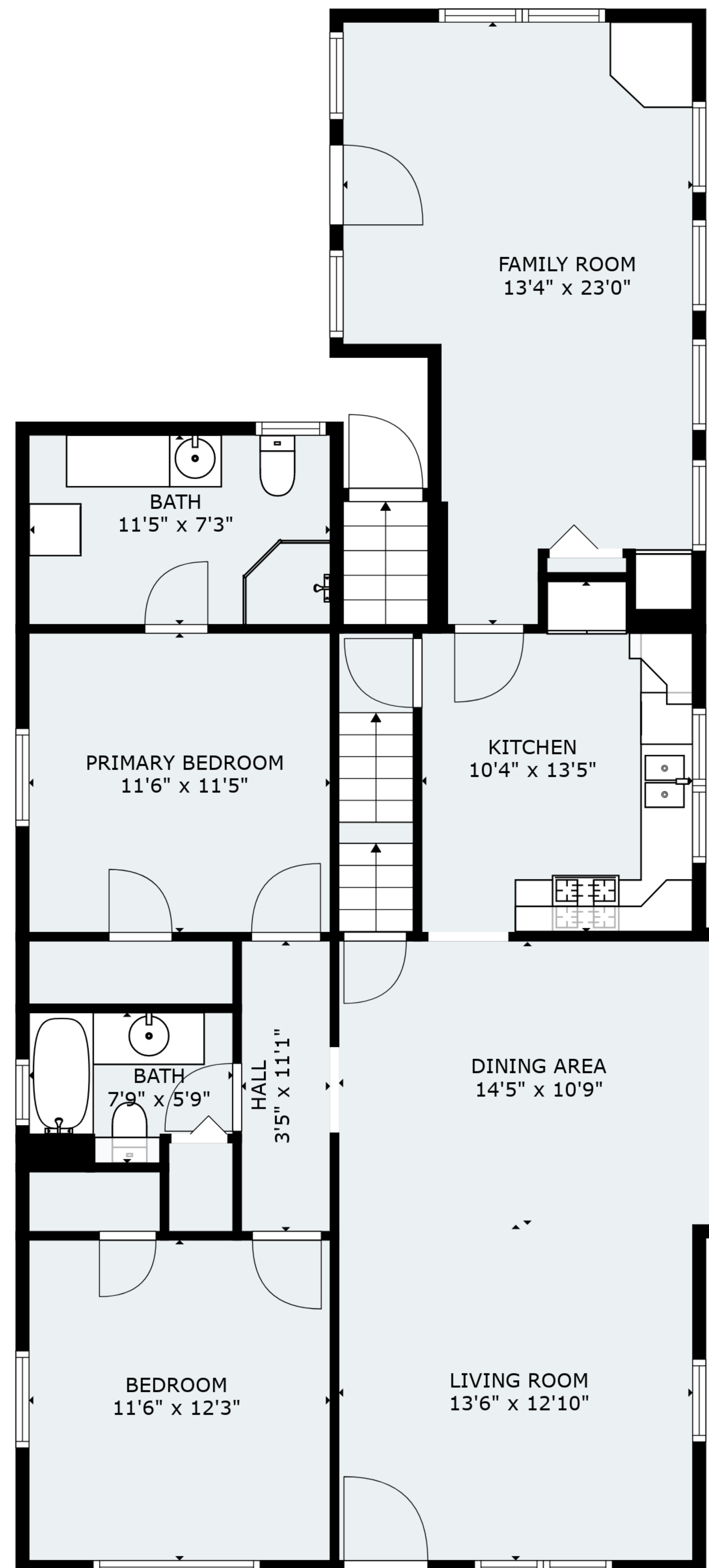
FLOOR 2
