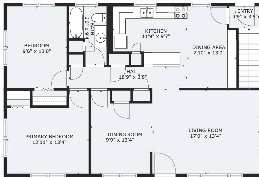
FLOOR 2
