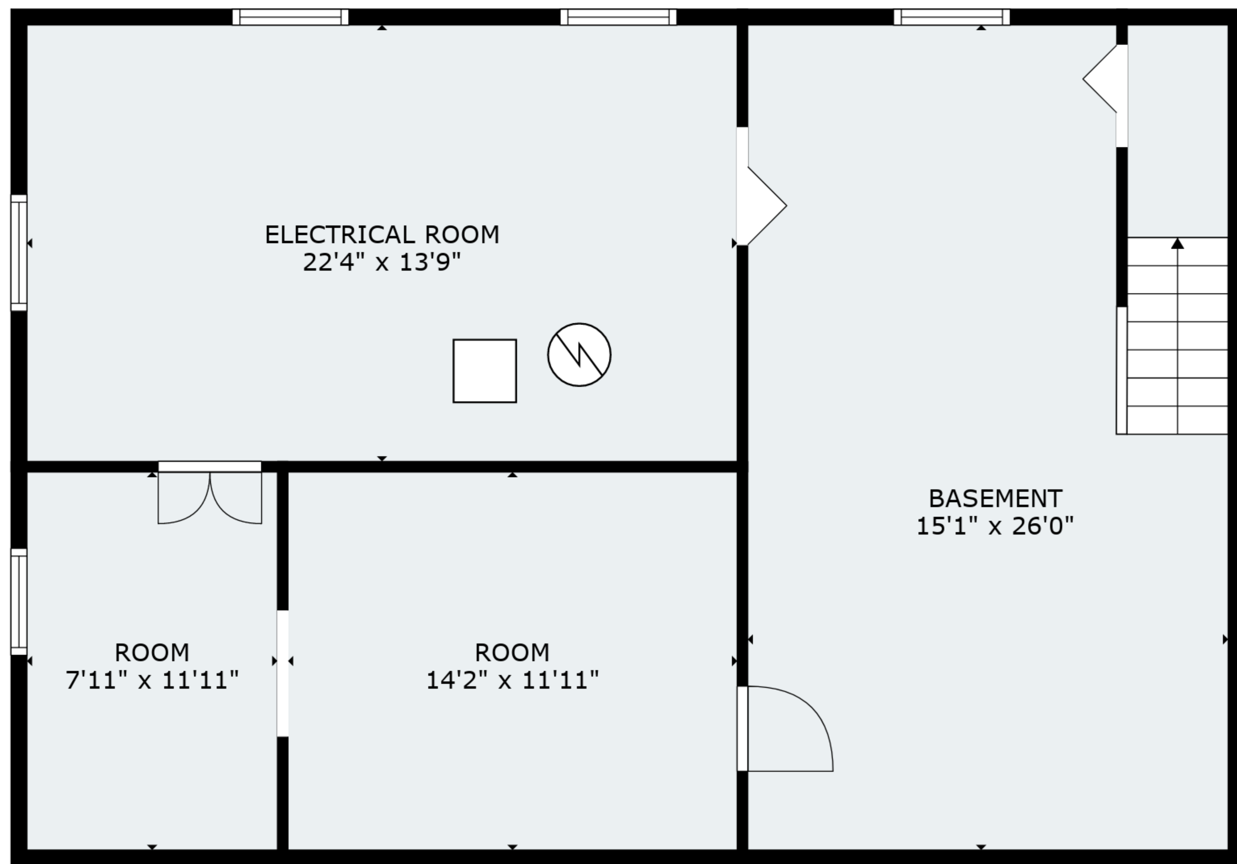
FLOOR 1
