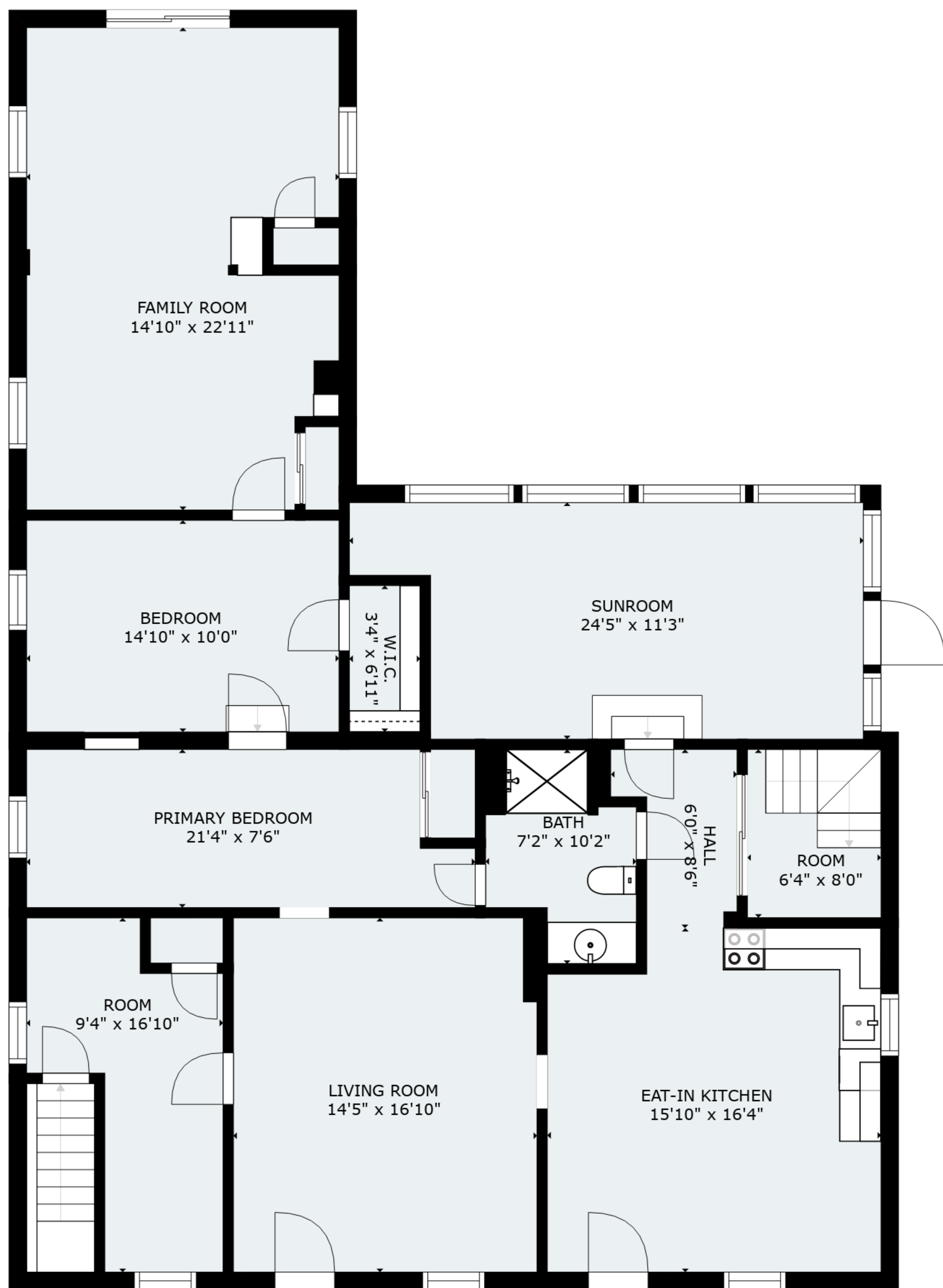
FLOOR 2
