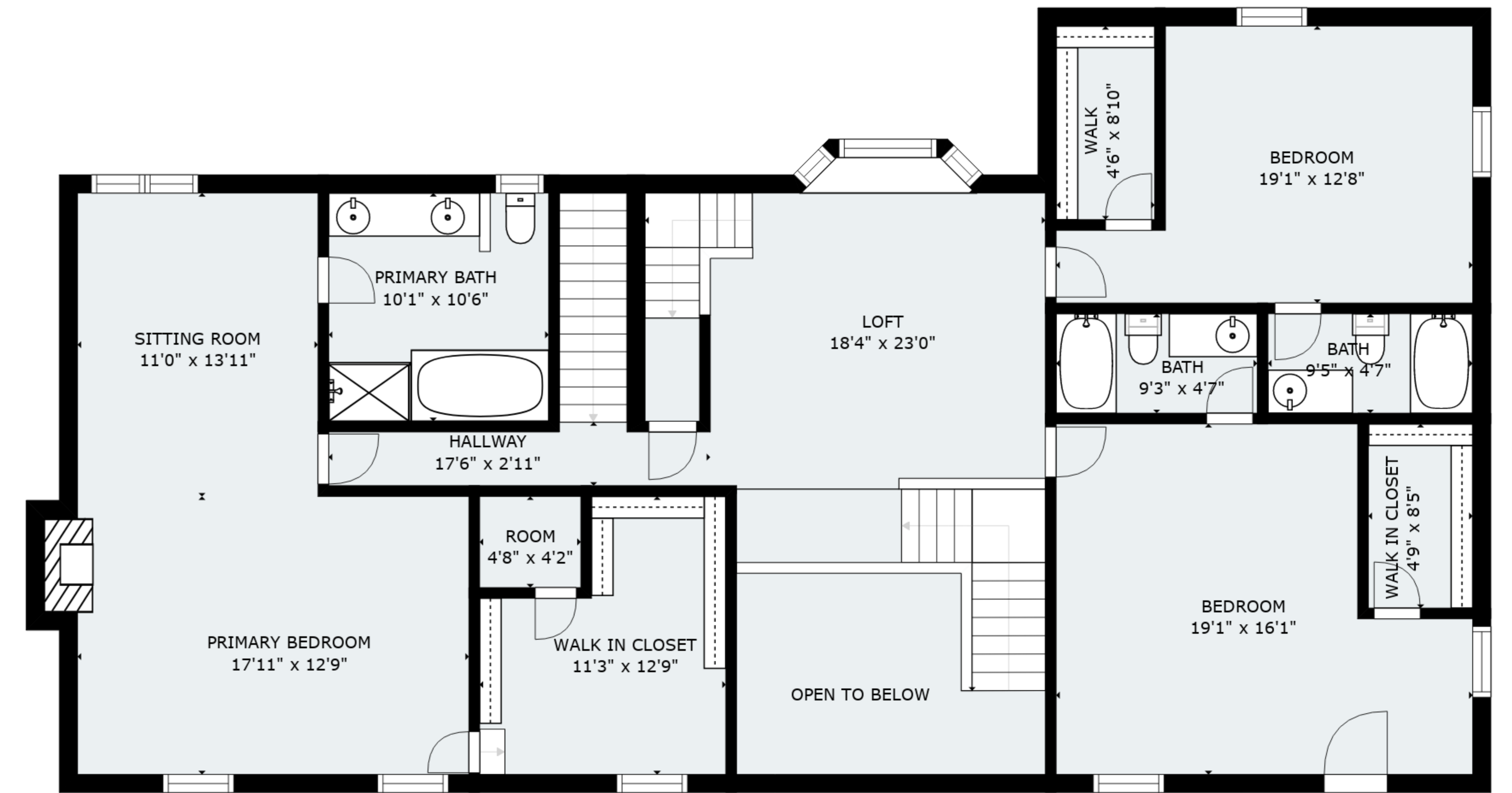
FLOOR 3
