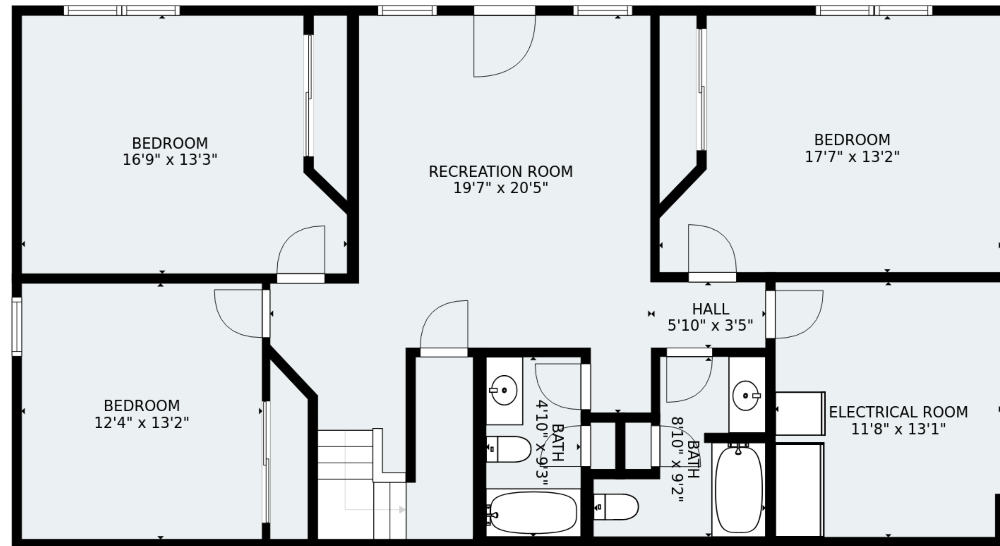
FLOOR 1
